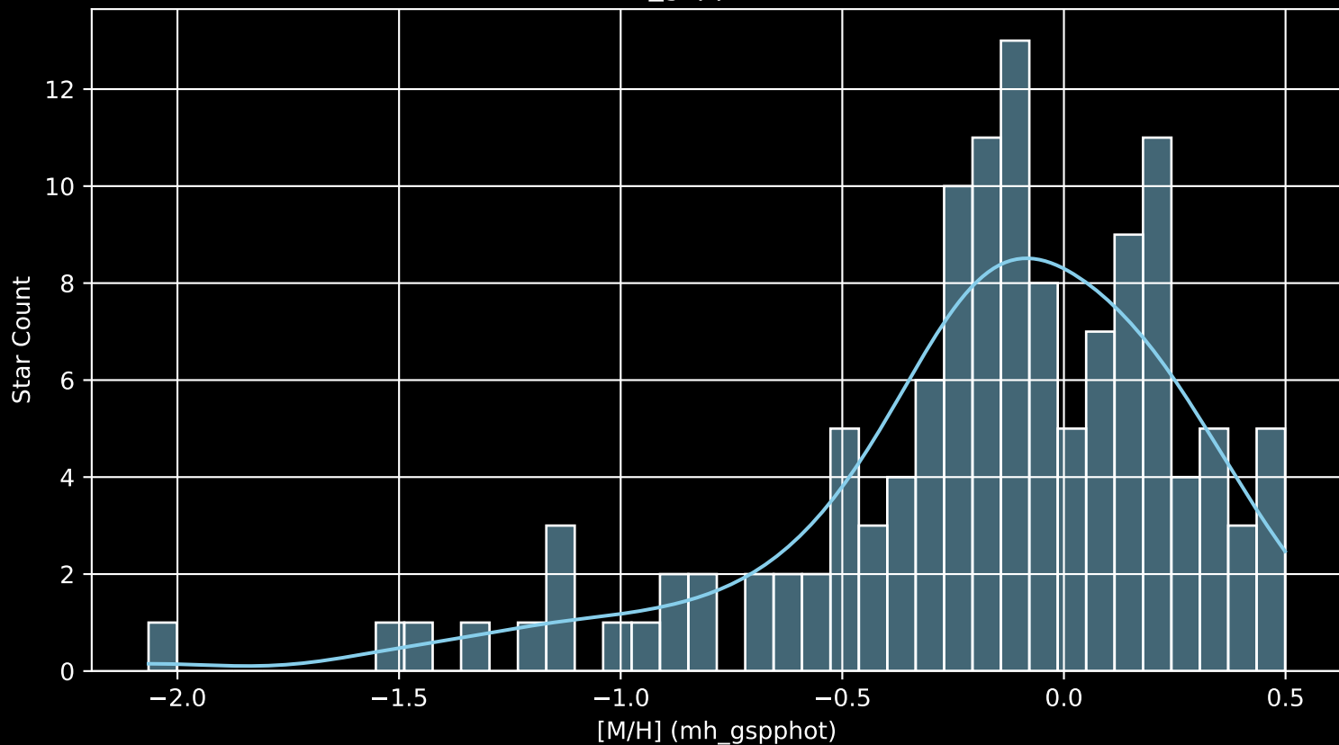
APOGEE DR17 Field: [278-31-O_TESS [M/H] (mh_gspphot) (n= 129)
