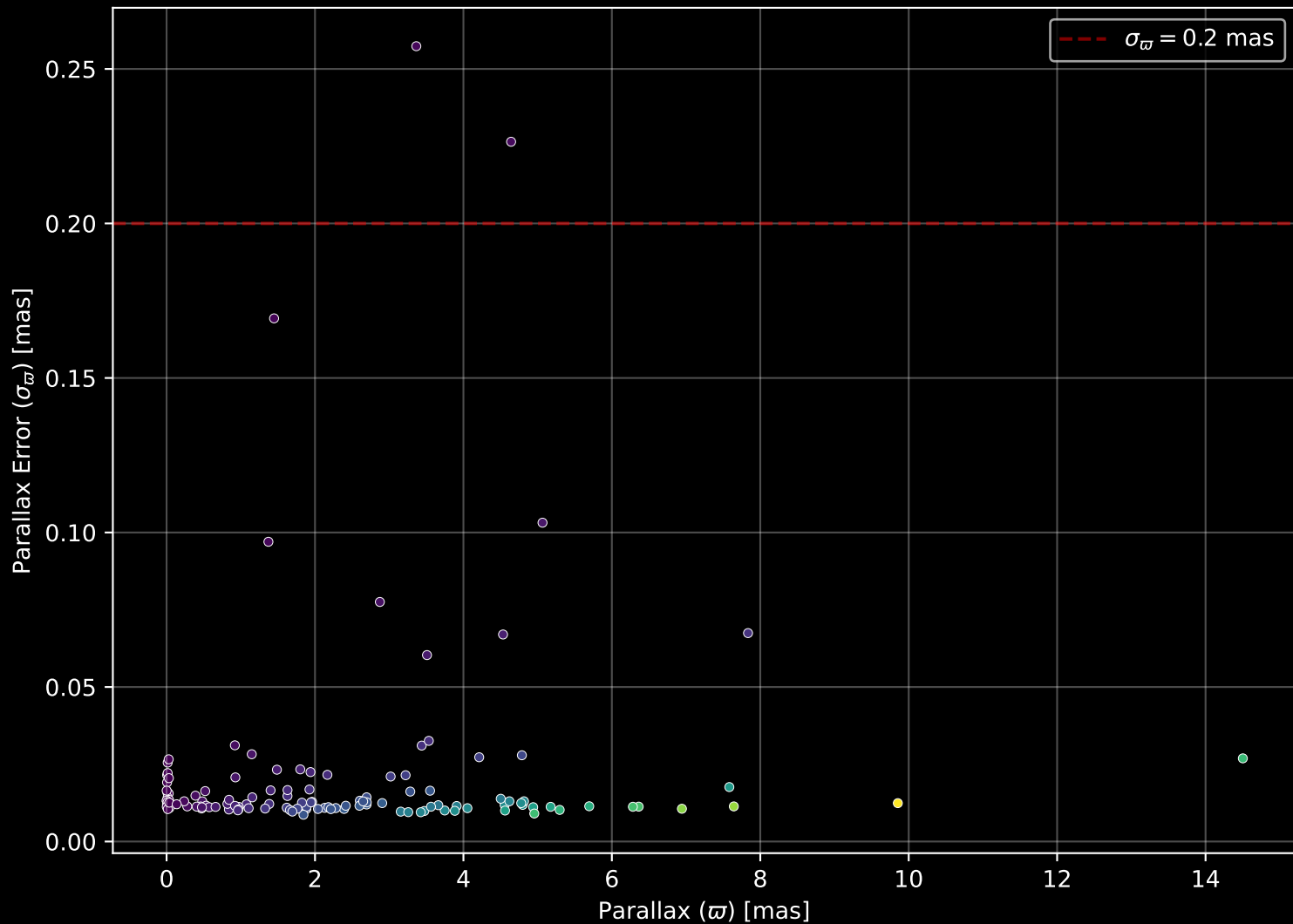
APOGEE DR17 Field: [278-31-O_TESS] Parallax Quality (n= 131)
