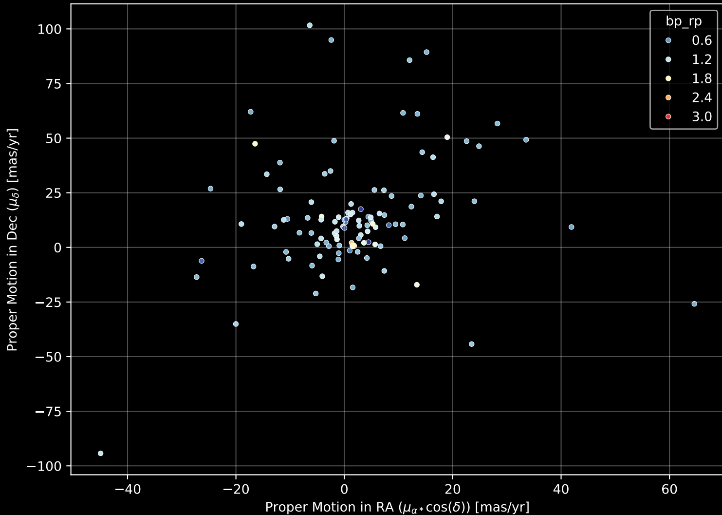
APOGEE DR17 Field: [278-31-O_TESS] Proper Motion Diagram (n= 131)
