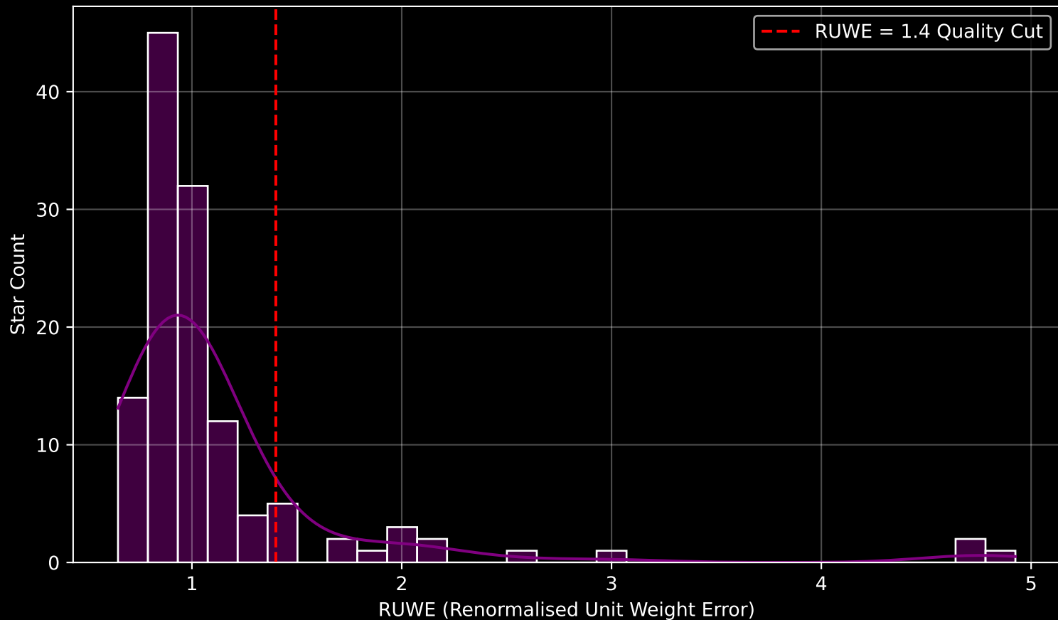
GAPOGEE DR17 Field [278-31-O_TESS] RUWE Distribution (n= 125)
