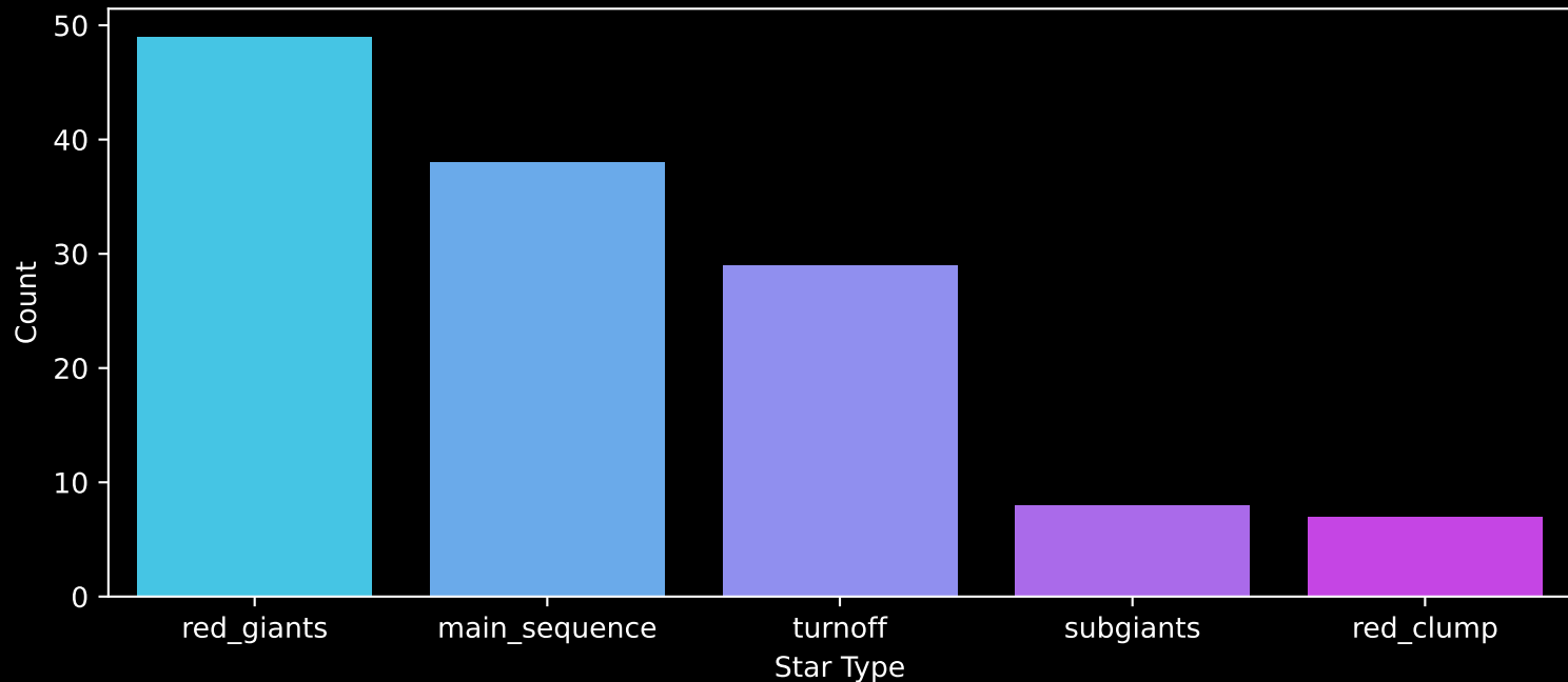
APOGEE DR17 Field: [278-31-O_TESS] Count plot of Star Type
