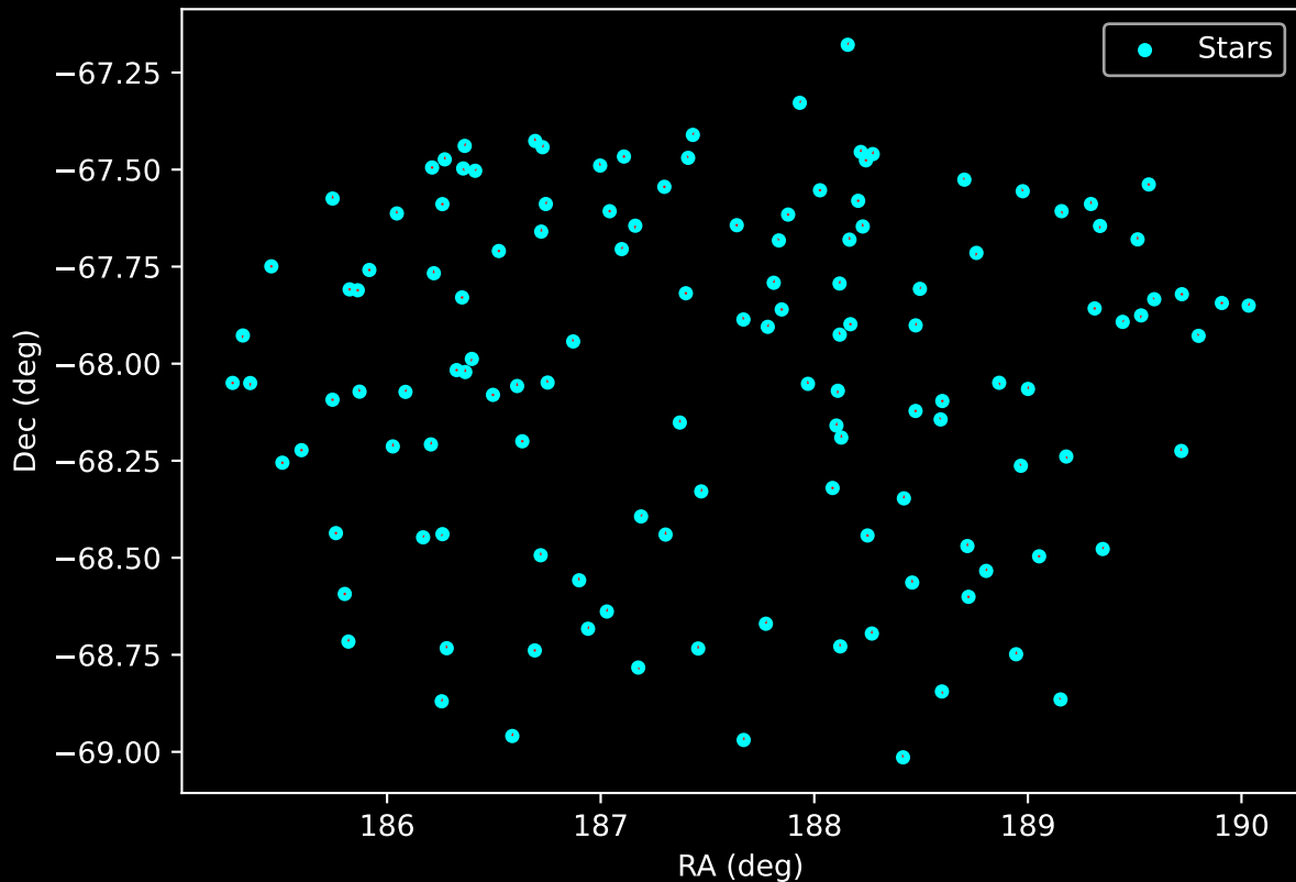
APOGEE DR17 Field: [278-31-O_TESS] Proper Motion Vectors for Gaia Star Field (n= 131)
